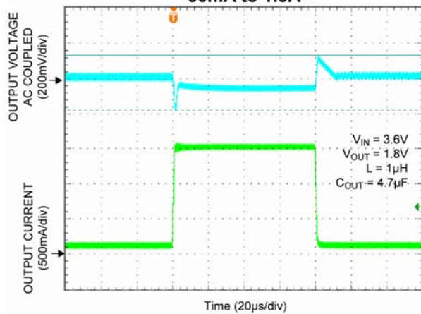
Load Transient 50mA to 1.5A
