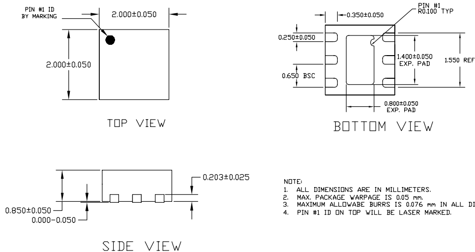
6 Pin 2mm x 2mm MLF (ML)
