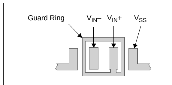
FIGURE 4-5: Example Guard Ring Layout for Inverting Gain.
