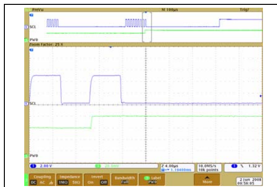
FIGURE 2-15: 5 k \Omega – Low-Voltage Increment Wiper Settling Time ( V_{DD} = 5.5\text{V} ) ( 1\text{ }\mu\text{s/Div} ).
