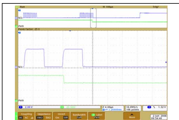
FIGURE 2-13: 5 k \Omega – Low-Voltage Decrement Wiper Settling Time ( V_{DD} = 2.7\text{V} ) ( 1\text{ }\mu\text{s/Div} ).
