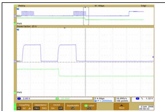
FIGURE 2-12: 5 k \Omega – Low-Voltage Decrement Wiper Settling Time ( V_{DD} = 5.5\text{V} ) ( 1\text{ }\mu\text{s/Div} ).
