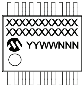
20-Lead SSOP
