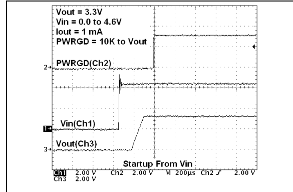
FIGURE 2-27: Power-up Timing.
