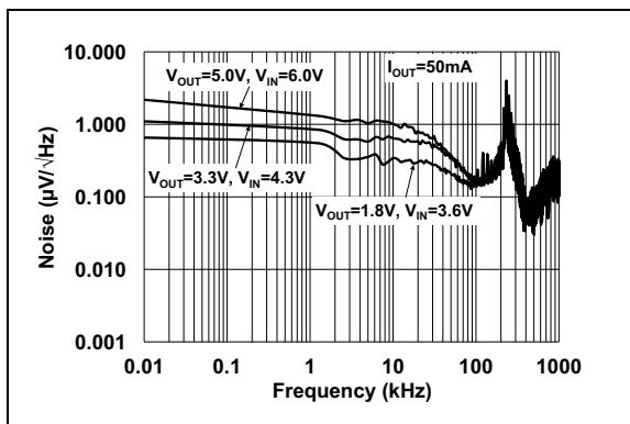
FIGURE 2-26: Output Noise vs. Frequency (three lines, V_R = 1.2\text{V} , 3.3\text{V} , 5.0\text{V} ).
