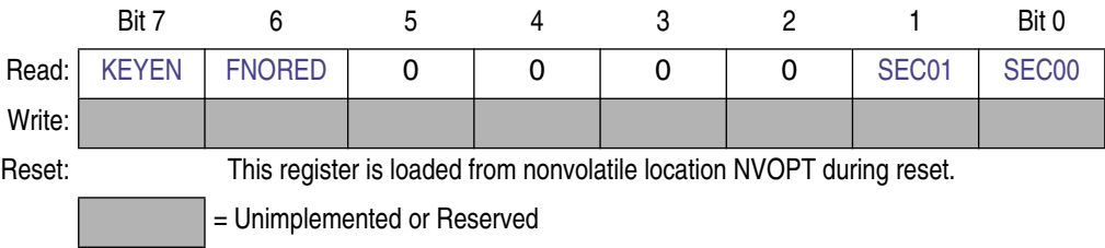
Figure 4-5. FLASH Options Register (FOPT)
