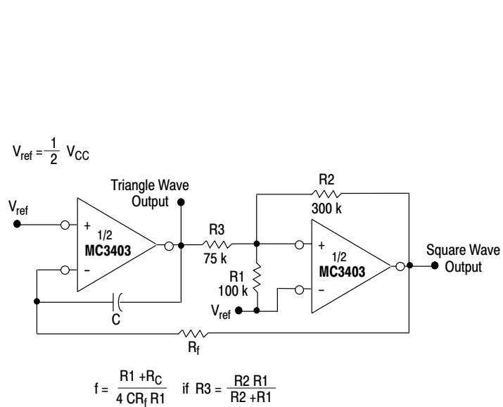
Figure 14. Function Generator
