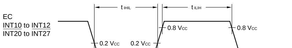
Peripheral Input Timing Diagram
