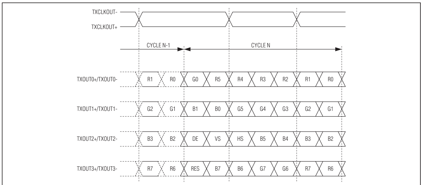
Figure 13. Typical Panel Clock and Bit Assignment
