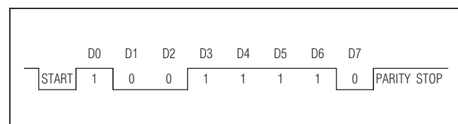
Figure 18. SYNC Byte (0x79)
