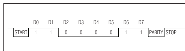
Figure 19. ACK Byte (0xC3)
