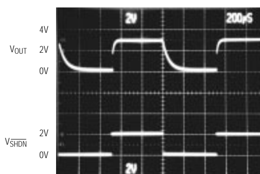
MAX8874 SHUTDOWN
