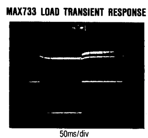
A: V_{OUT} , 50mV/div, DC-Coupled B: I_{OUT} , 50mA/div, 10mA to 125mA Circuit of Fig. 2, V_+ = +6\text{V} , T_A = +25^{\circ}\text{C}
