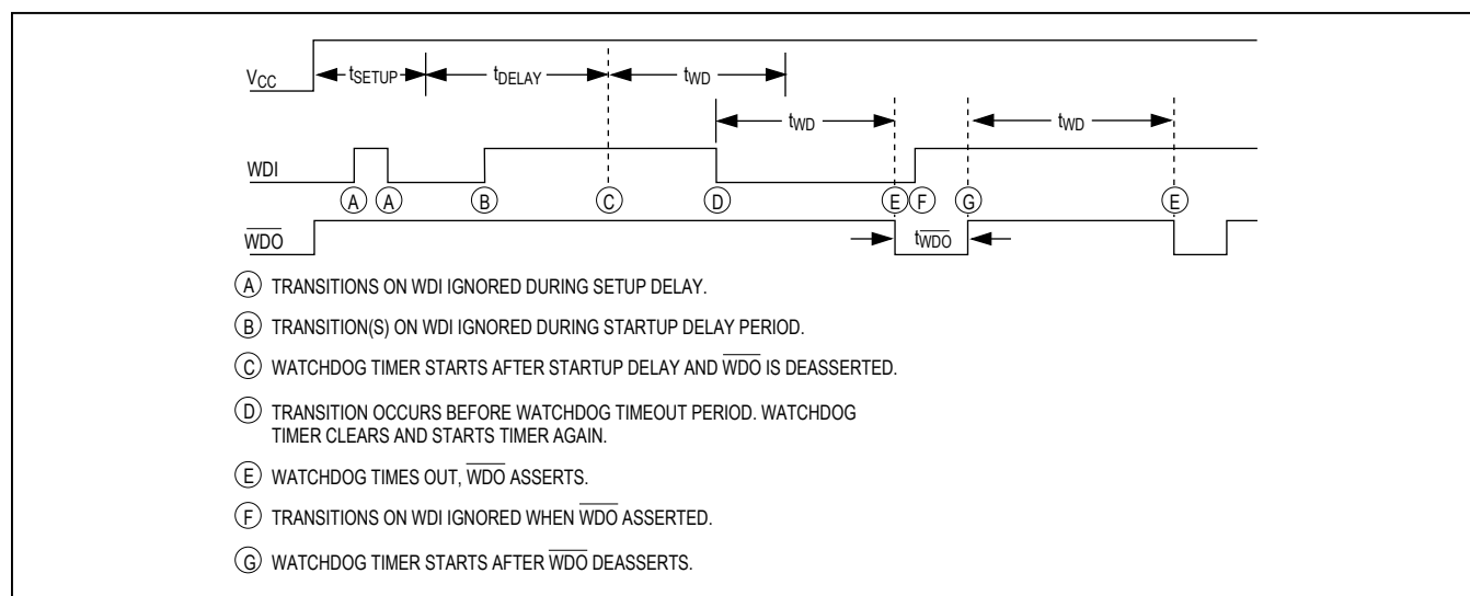
Figure 1. Watchdog Timing
