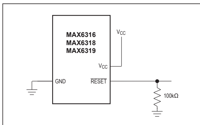
Figure 8. Ensuring \overline{\text{RESET}} Valid to VCC = 0V on Active-Low Push/Pull and Bidirectional Outputs
