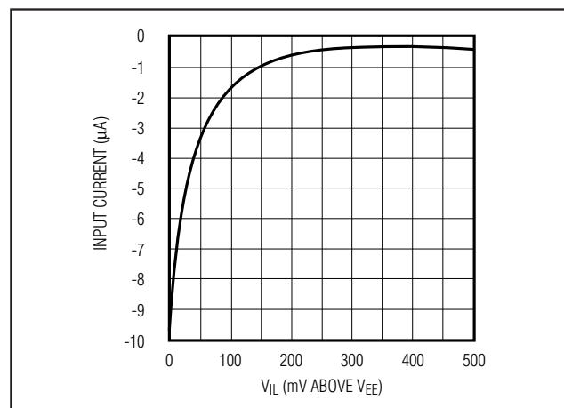
Figure 4. Enable Logic-Low Input Current vs. Enable Logic-Low Threshold with 10\text{k}\Omega Series Resistor
