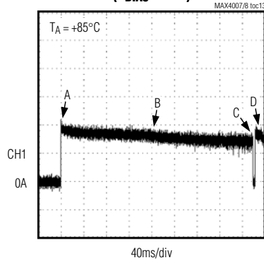
SHORT-CIRCUIT RESPONSE ( V_{\text{BIAS}} = 76\text{V} )
