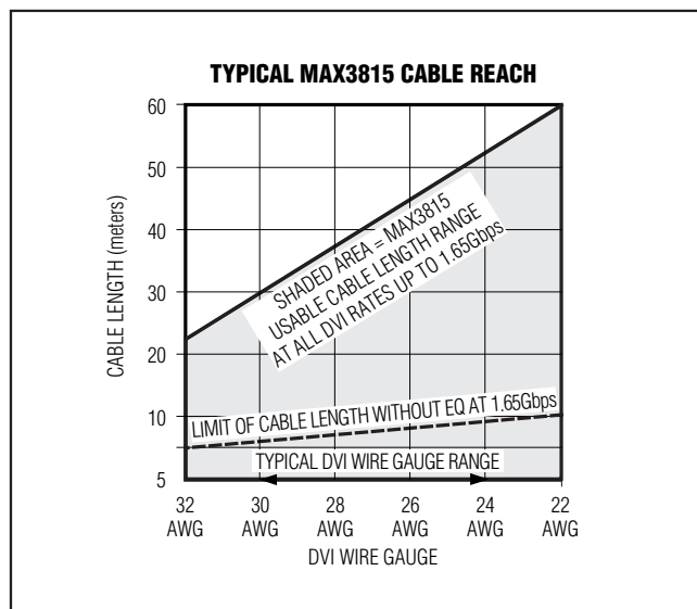
Figure 6. Cable Reach
