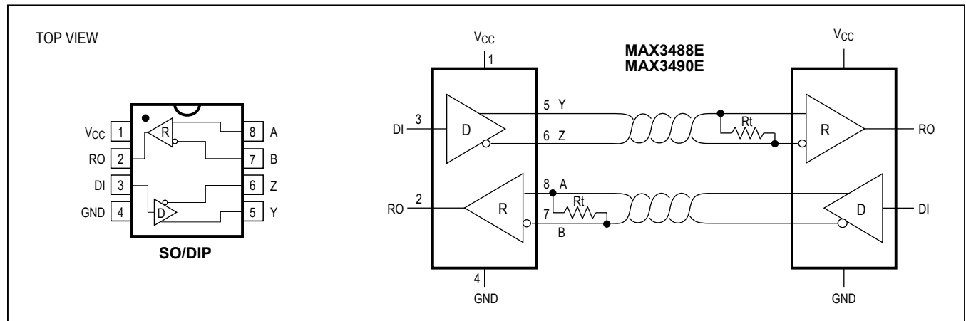
Figure 2. MAX3488E/MAX3490E Pin Configuration and Typical Operating Circuit
