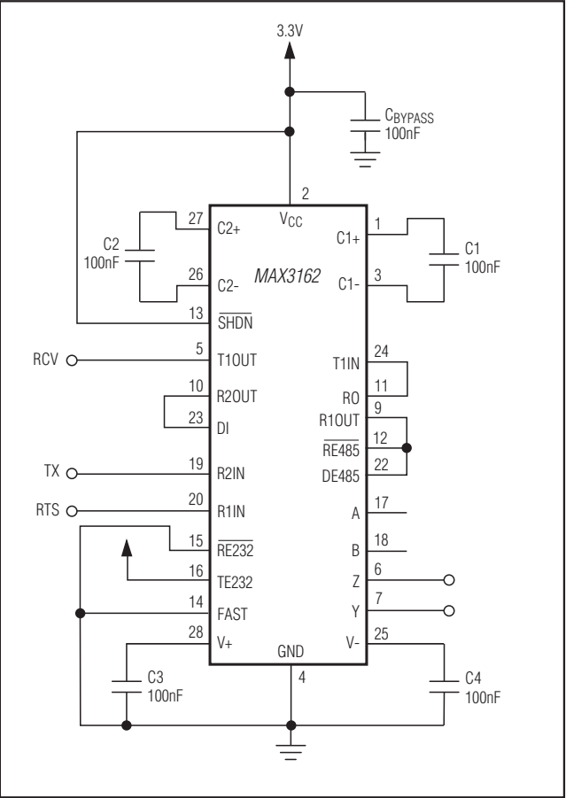
Figure 15. Protocol Translator
