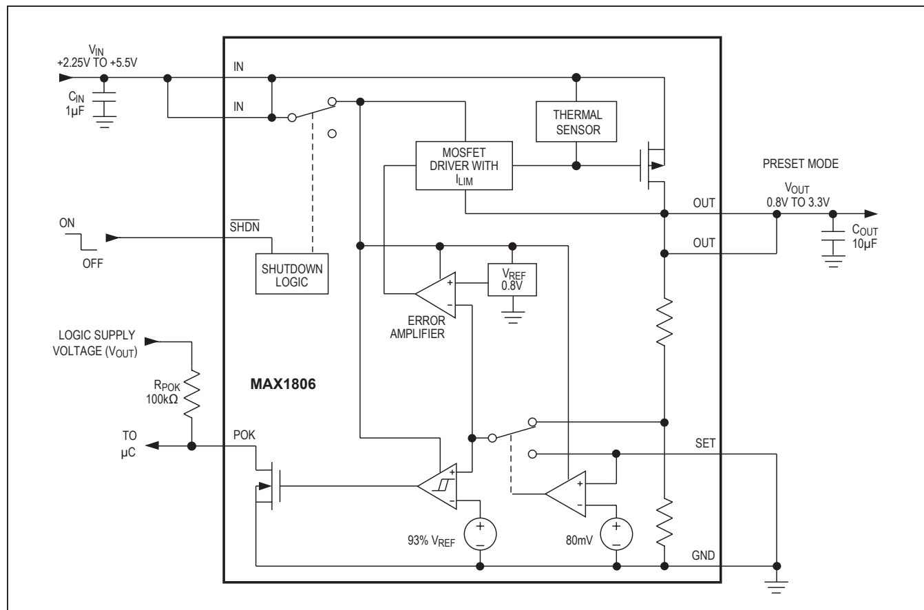
Figure 1. Functional Diagram
