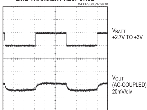
LINE-TRANSIENT RESPONSE
