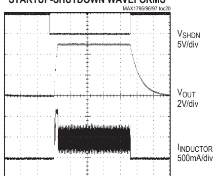
STARTUP-SHUTDOWN WAVEFORMS
