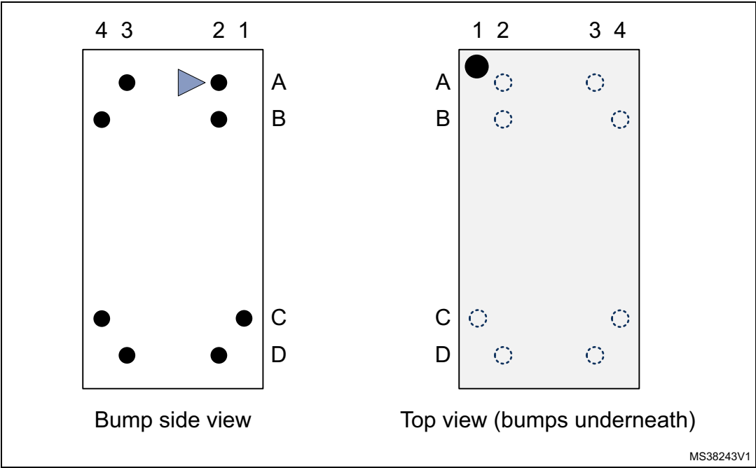
Figure 3. WLCSP connections
