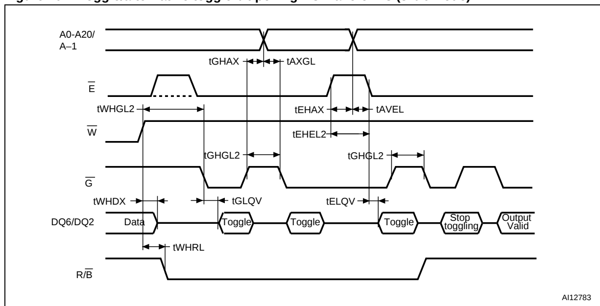
Figure 20. Toggle/alternative toggle bit polling AC waveforms (8-bit mode)
