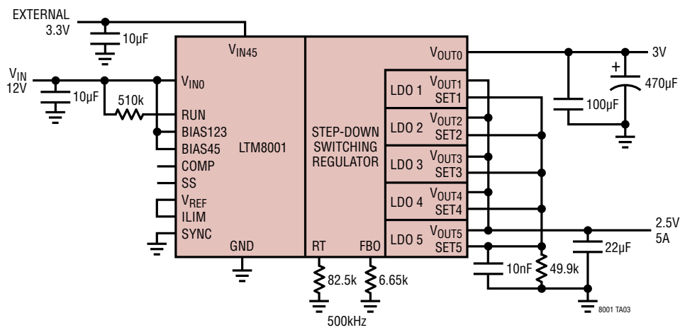
Dual Input, 2.5V 5A DC/DC \mu Module Converter Using a Single LTM8001 (External 3.3V Turns On Before or Simultaneously with 12V)
