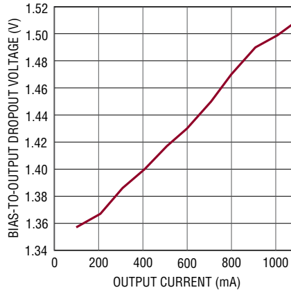
LDO V_{\text{BIAS}} -to-Output Dropout Voltage vs Output Current
