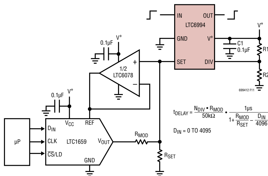
Figure 11. Digitally Controlled Delay
