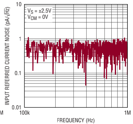
Input Referred Current Noise vs Frequency
