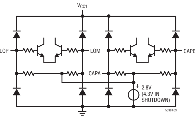
Figure 3. Simplified Circuit Schematic for the LOP, LOM, CAPA and CAPB Inputs.
