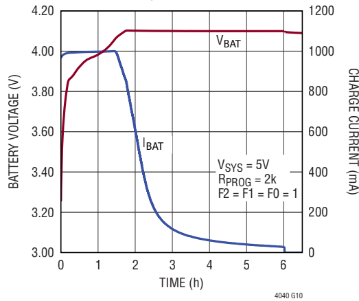
Li-Ion Battery Charging Profile
