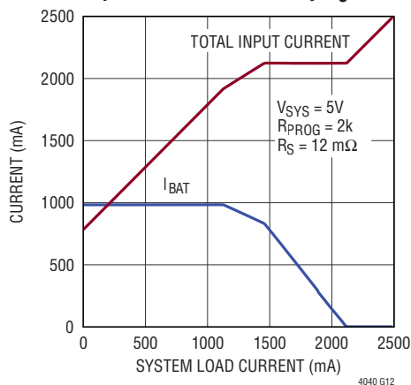
Charge Current Reduction Due to Input Current Limit Set by R_S
