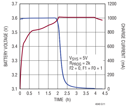
LiFePO 4 Battery Charging Profile
