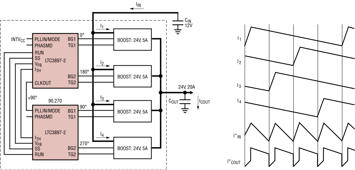
4-Phase 480W Single Output Boost Regulator
