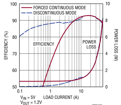
Figure 18. 4.5V to 14V Input, 1.2V/50A 2-Phase Single Output, 300kHz, DCR Sense, DTR Enabled, Step-Down Converter
