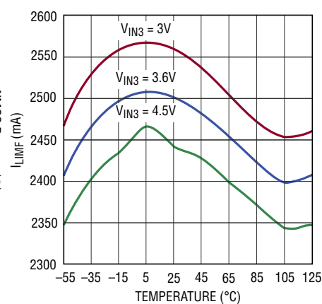
Buck-Boost Regulator Forward Current Limit
