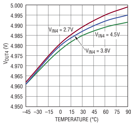
Boost Output Voltage vs Temperature
