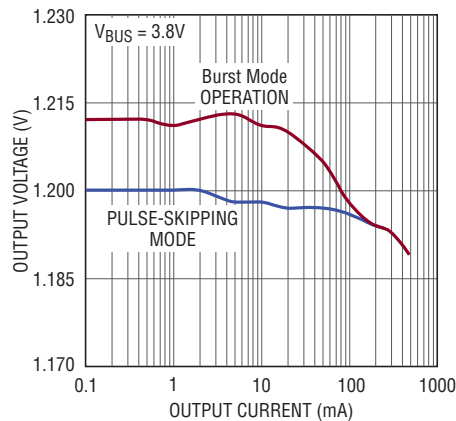
Switching Regulators 1, 2 Load Regulation at V_{OUT1,2} = 1.2\text{V}
