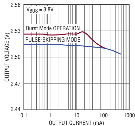
Switching Regulators 1, 2 Load Regulation at V_{OUT1,2} = 2.5\text{V}
