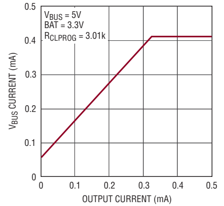
V_{BUS} Current vs Output Current in Suspend
