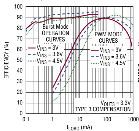
Buck-Boost Regulator Efficiency vs I_{LOAD}
