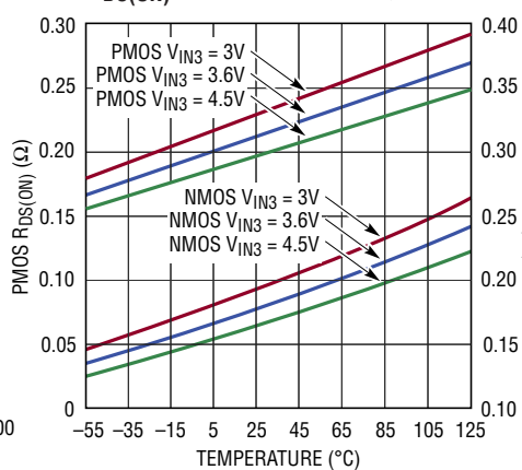
R_{DS(ON)} For Buck-Boost Regulator
