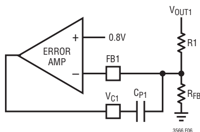
Figure 6. Error Amplifier with Type I Compensation
