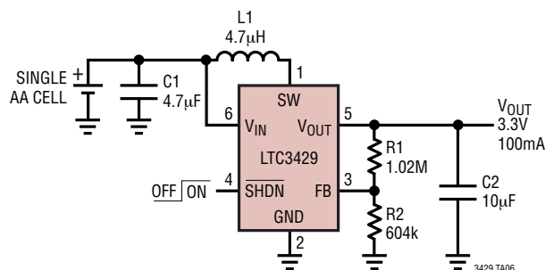
Single AA Cell to 3.3V
