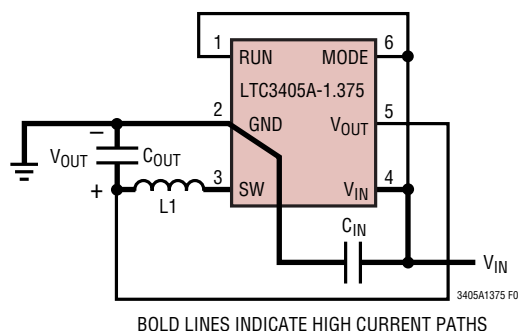
Figure 3. LTC3405A-1.375 Layout Diagram
