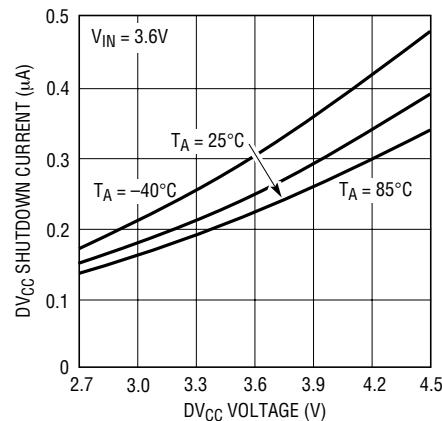
DV_{\text{CC}} Shutdown Current vs Input Voltage
