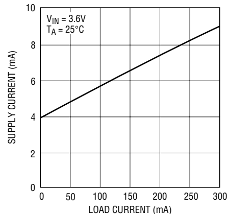
1.5x Mode Supply Current vs I_{\text{CPO}} ( I_{\text{IN}} = 1.5I_{\text{CPO}} )
