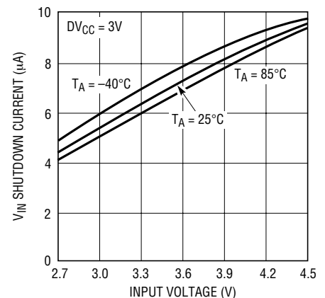
V_{\text{IN}} Shutdown Current vs Input Voltage
