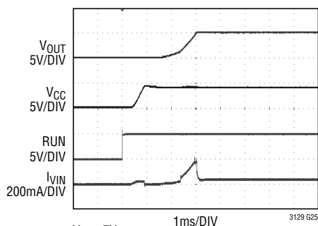
Start-Up Waveforms
