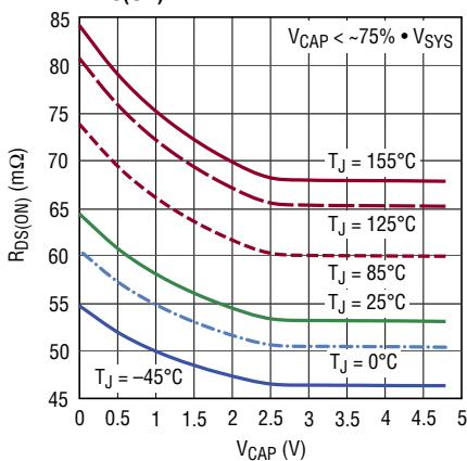
R_{DS(ON)} of SWA Static
