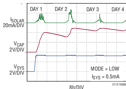
Charging with Solar Current and 24/7 Backup
