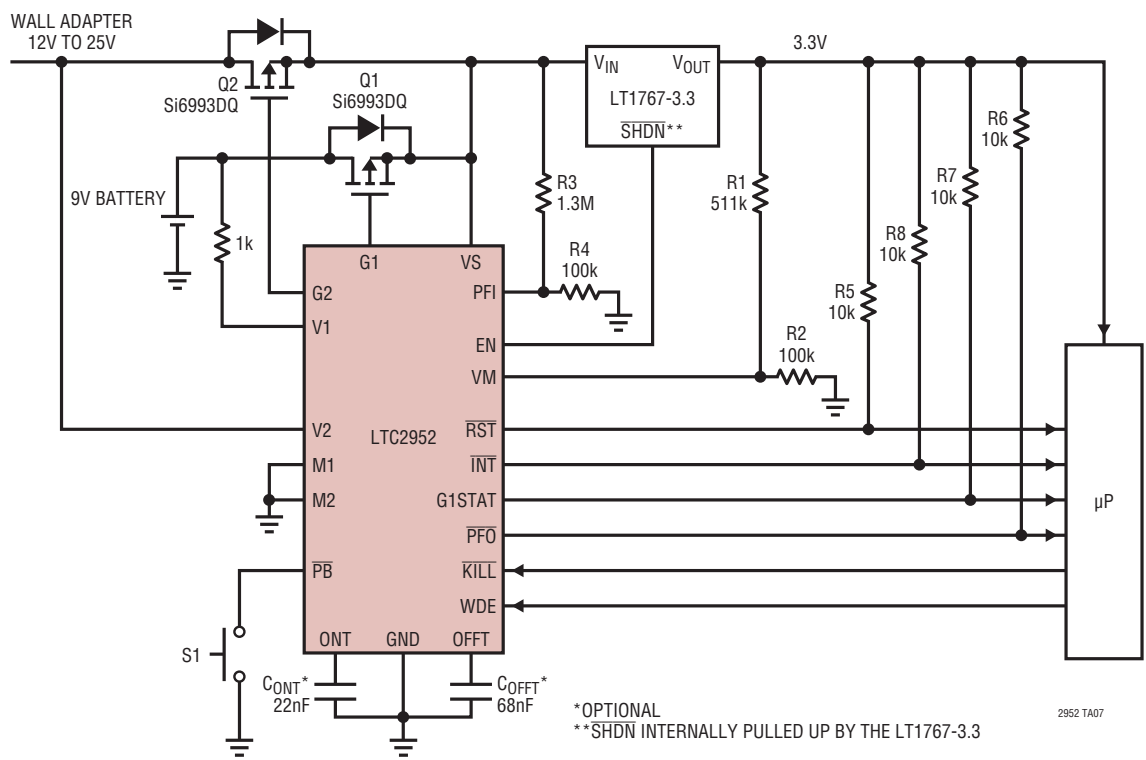
Wall Adapter and Battery Automatic Load Switchover with Reverse Battery Protection
