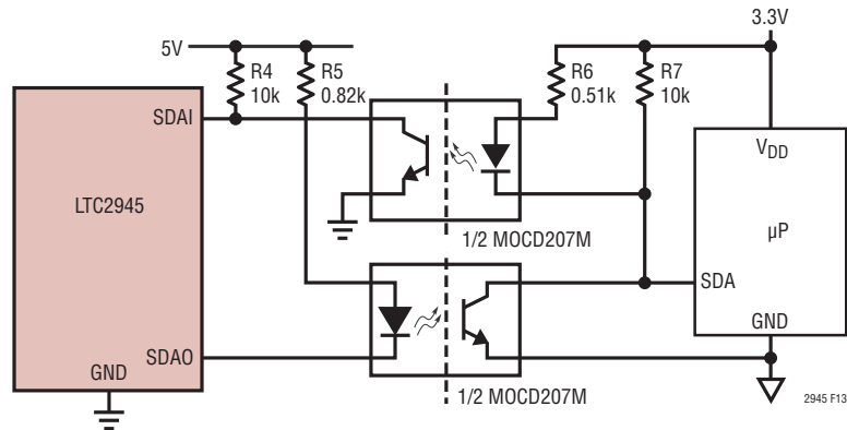
Figure 13. Opto-Isolation of a 10kHz I²C Interface Between LTC2945 and Microcontroller (SCL Omitted for Clarity)
