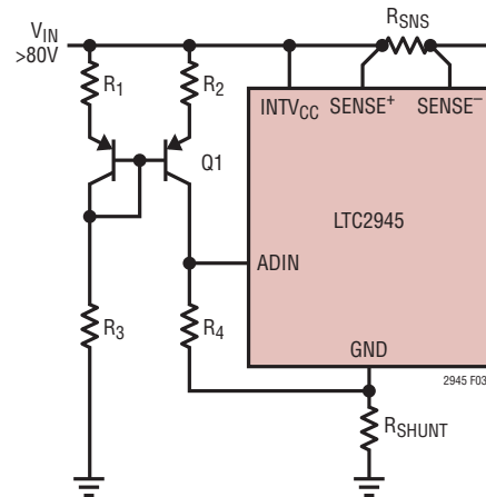
Figure 3a. LTC2945 Derives Power Through High-Side Shunt Regulator
