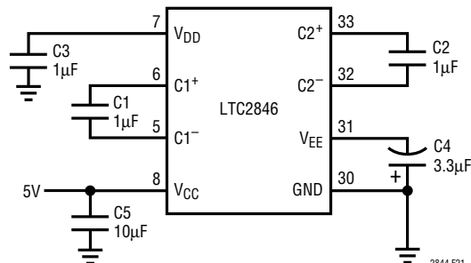
Figure 21. Charge Pump
