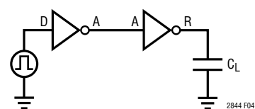
Figure 4. V.10/V.28 Receiver Test Circuit
