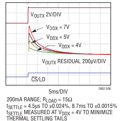
Settling 0 to 200mA Step
