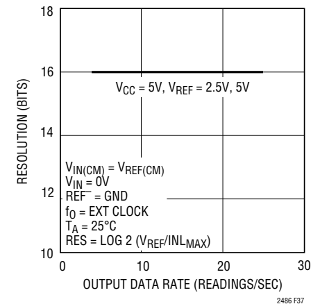
Figure 37. Resolution (INL MAX ≤ 1LSB) vs Output Data Rate and Reference Voltage
