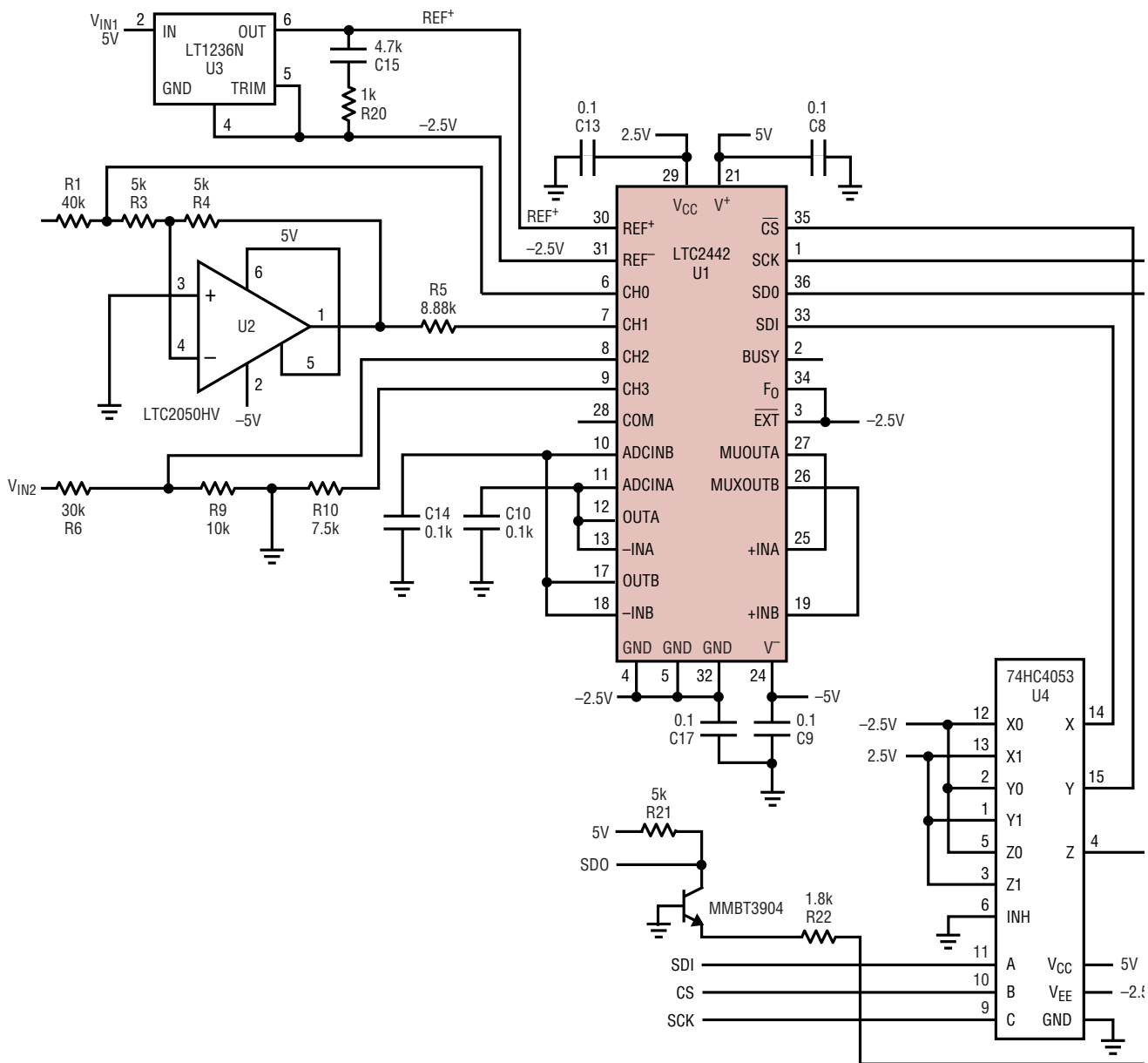
Figure 20. Scaling Inputs for \pm 10\text{V} Range
