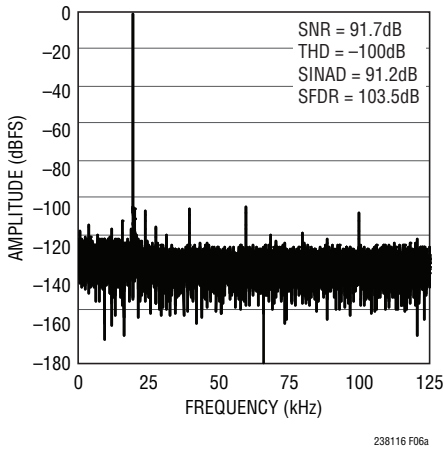
Figure 6a. 32k Point FFT Plot for Circuit Shown in Figure 6
