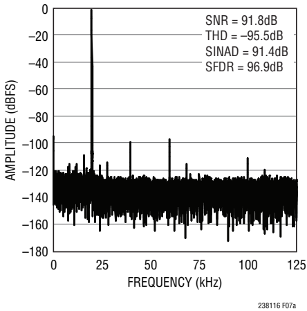
Figure 7a. 32k Point FFT Plot for Circuit Shown in Figure 7
