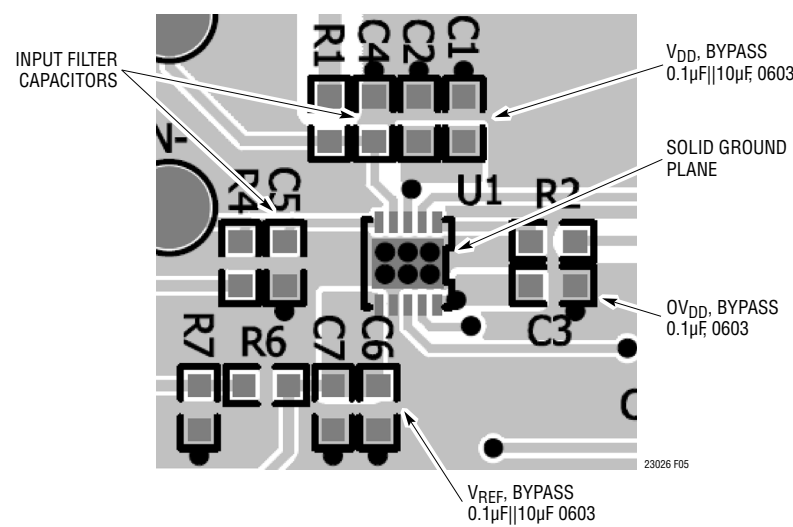
Figure 5. Suggested Layout
