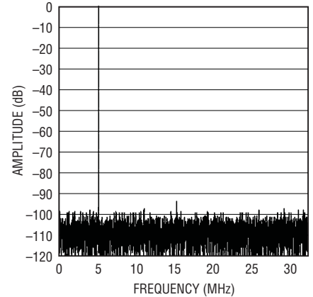
LTC2228: 8192 Point FFT, f_{IN} = 5\text{MHz} , -1dB, 2V Range, 65Msps
