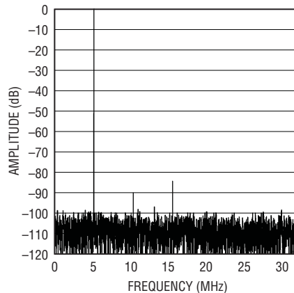
LTC2228: 8192 Point FFT, f_{IN} = 70\text{MHz} , -1dB, 2V Range, 65Msps
