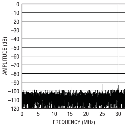
LTC2228: 8192 Point FFT, f_{IN} = 30\text{MHz} , -1dB, 2V Range, 65Msps
