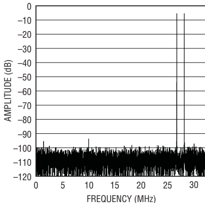
LTC2228: 8192 Point 2-Tone FFT, f_{IN} = 28.2\text{MHz} and 26.8\text{MHz} , -1dB, 2V Range, 65Msps
