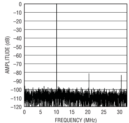
LTC2228: 8192 Point FFT, f_{IN} = 140\text{MHz} , -1dB, 2V Range, 65Msps
