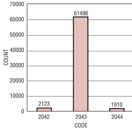
LTC2228: Grounded Input Histogram, 65Msps
