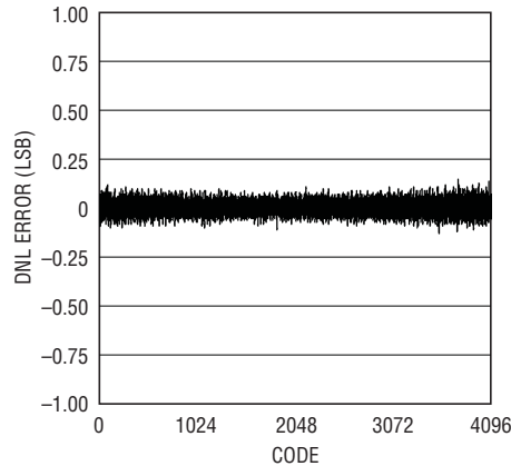
LTC2228: Typical DNL, 2V Range, 65Msps
