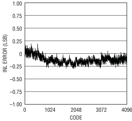
LTC2228: Typical INL, 2V Range, 65Msps
