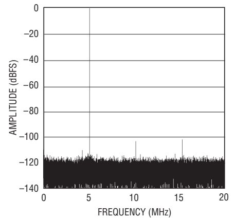
LTC2204: 64K Point FFT, 40Msps, f_{IN} = 5.1\text{MHz} , -1dBFS, PGA = 0, DITH = 0
