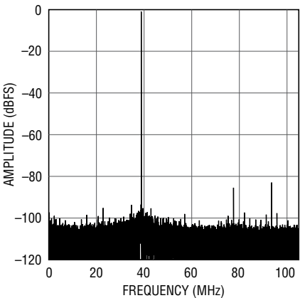
LTC2151-12: 32K Point FFT, f_{IN} = 171\text{MHz} , -1dBFS, 210Msps
