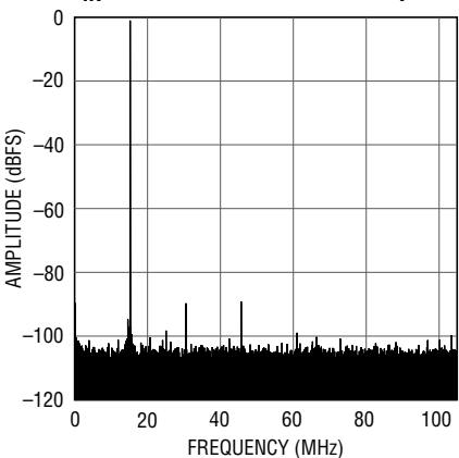
LTC2151-12: 32K Point FFT, f_{IN} = 15\text{MHz} , -1dBFS, 210Msps
