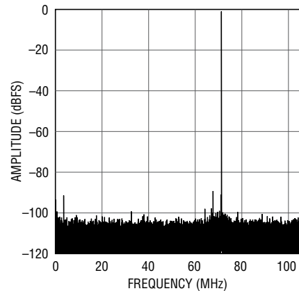
LTC2151-12: 32K Point FFT, f_{IN} = 71\text{MHz} , -1dBFS, 210Msps
