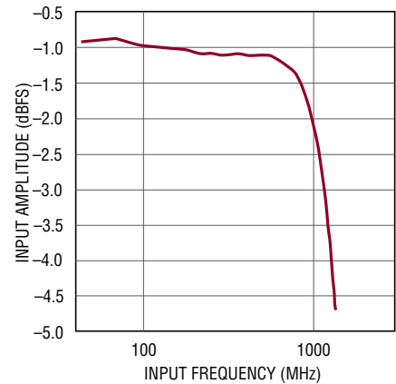
LTC2152-12: Frequency Response
