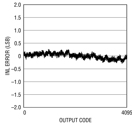
LTC2151-12: Integral Nonlinearity INL
