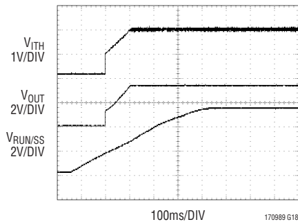
Soft-Start (Figure 12)
