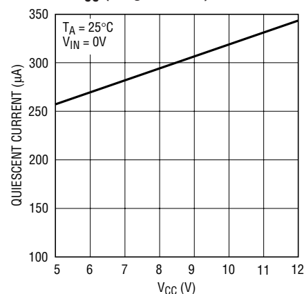
Quiescent Current vs V_{CC} (Single Driver)
